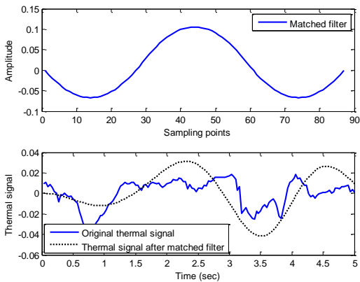
Fig 4: Passing thermal signal through matched filter: the upper is the designed matched filter and the lower is the comparison of thermal signals before and after matched filter.
