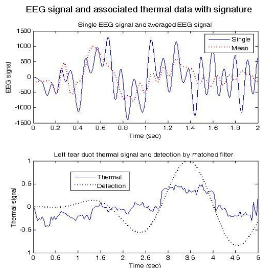
Fig 1: The EEG and thermal data from a subject that is concealing knowledge (subject instructed to conceal prior interaction with object): (A) The EEG data shows an average signal calculated over the subject's EEG signal, which shows a clear depiction of the P300 signal within the first second. (B) The thermal data shows a rise and return in temperature between the 3 rd and 4 th second (our signature of concealed knowledge).
